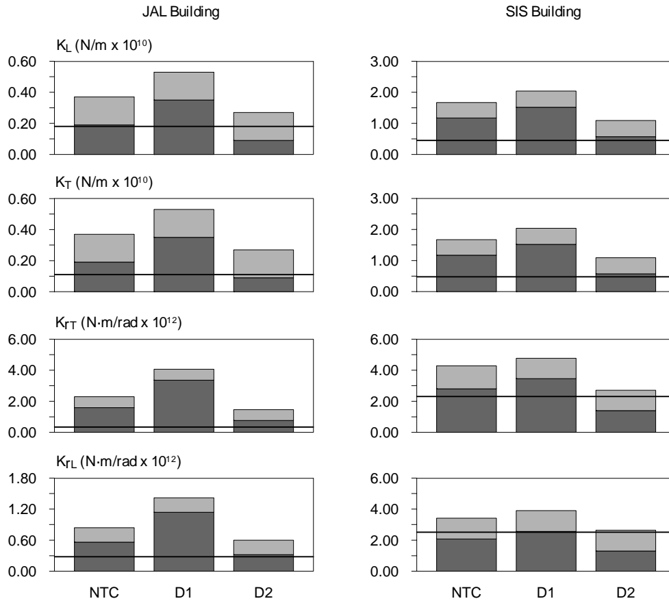
Figure 10. Estimated stiffnesses from analytical models and SIM method
