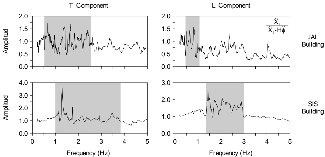
Figure 6. Rocking ( RT_R ) spectral ratios
