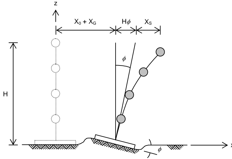
Figure 4. Simplified SSI model
