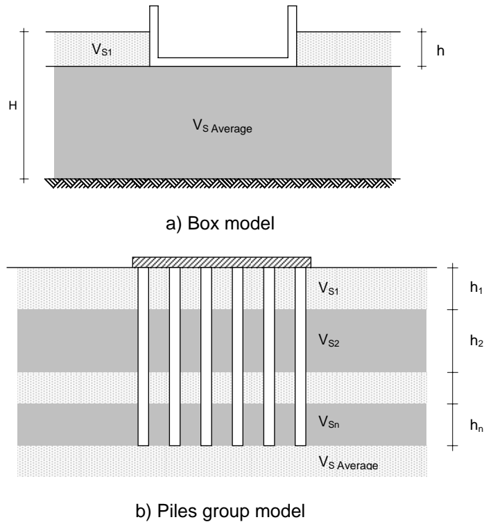
Figure 2. Basic models for assessment of foundation stiffnesses
