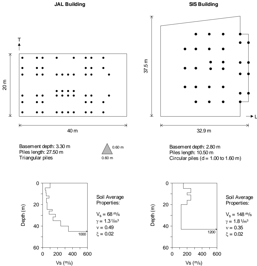
Figure 1. JAL and SIS building foundation plants and relevant soil properties
