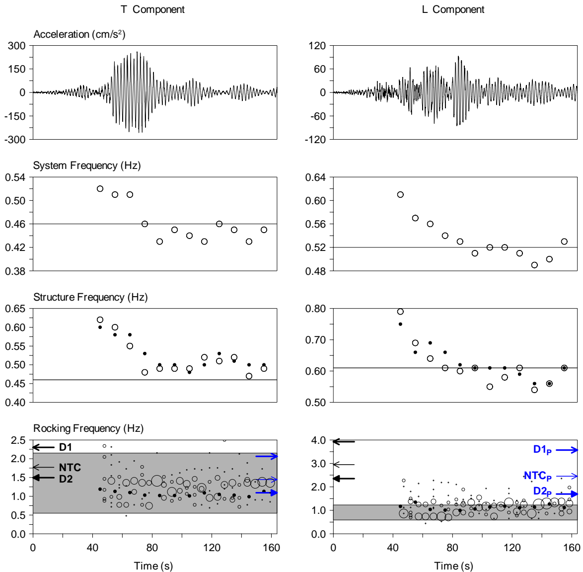
Figure 8. Identified and estimated frequencies for the JAL building
