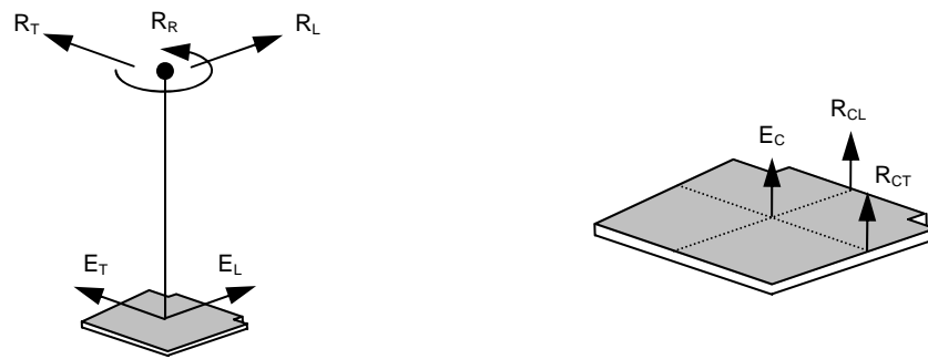
Figure 7. Fixed-base structure (left) and base rocking (right) models for SID method
