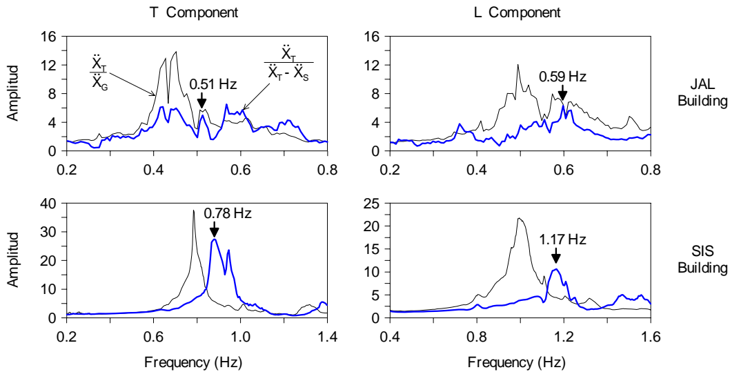
Figure 5. Fixed-base ( RF_s ) and system ( RF_{sys} ) spectral ratios
