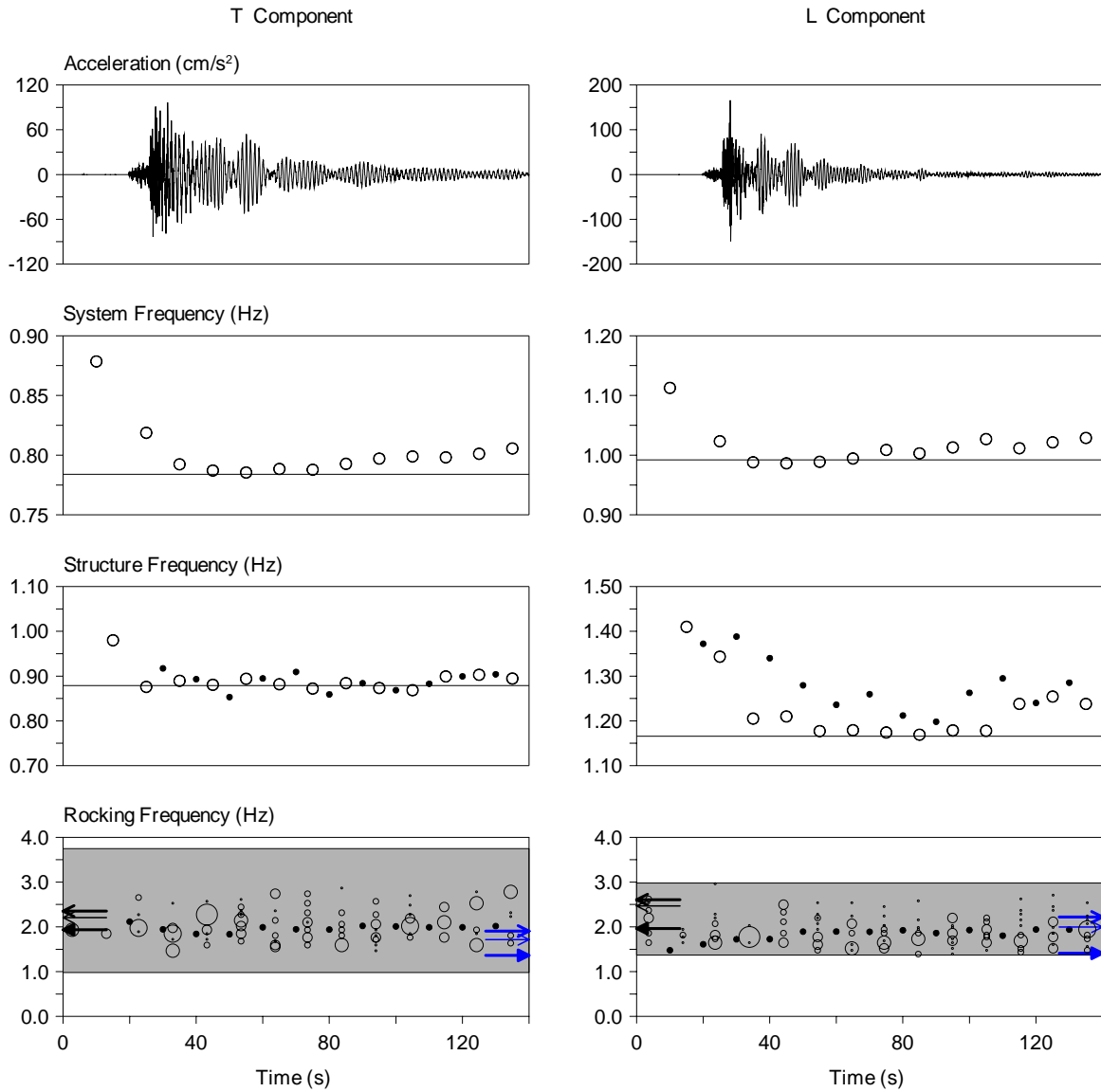
Figure 9. Identified and estimated frequencies for the SIS building
