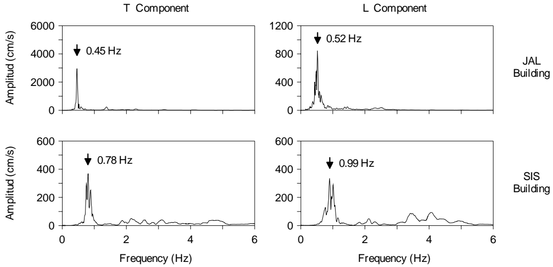
Figure 3. Fourier spectrum of recorded motions at the center of the roof
